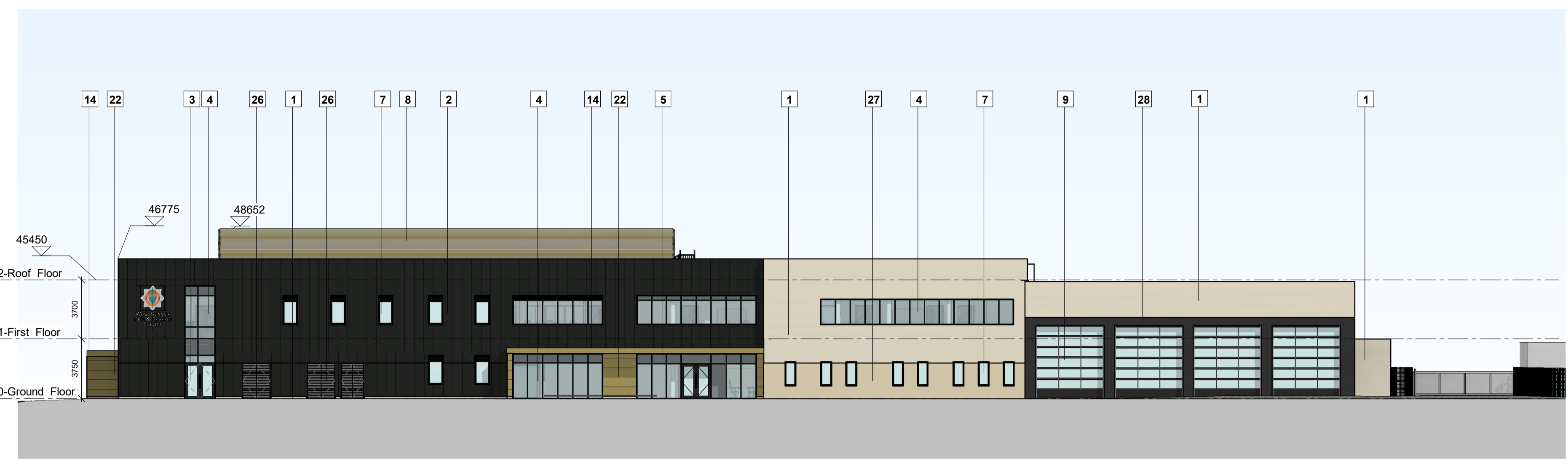
2 Elevation West 1:200
