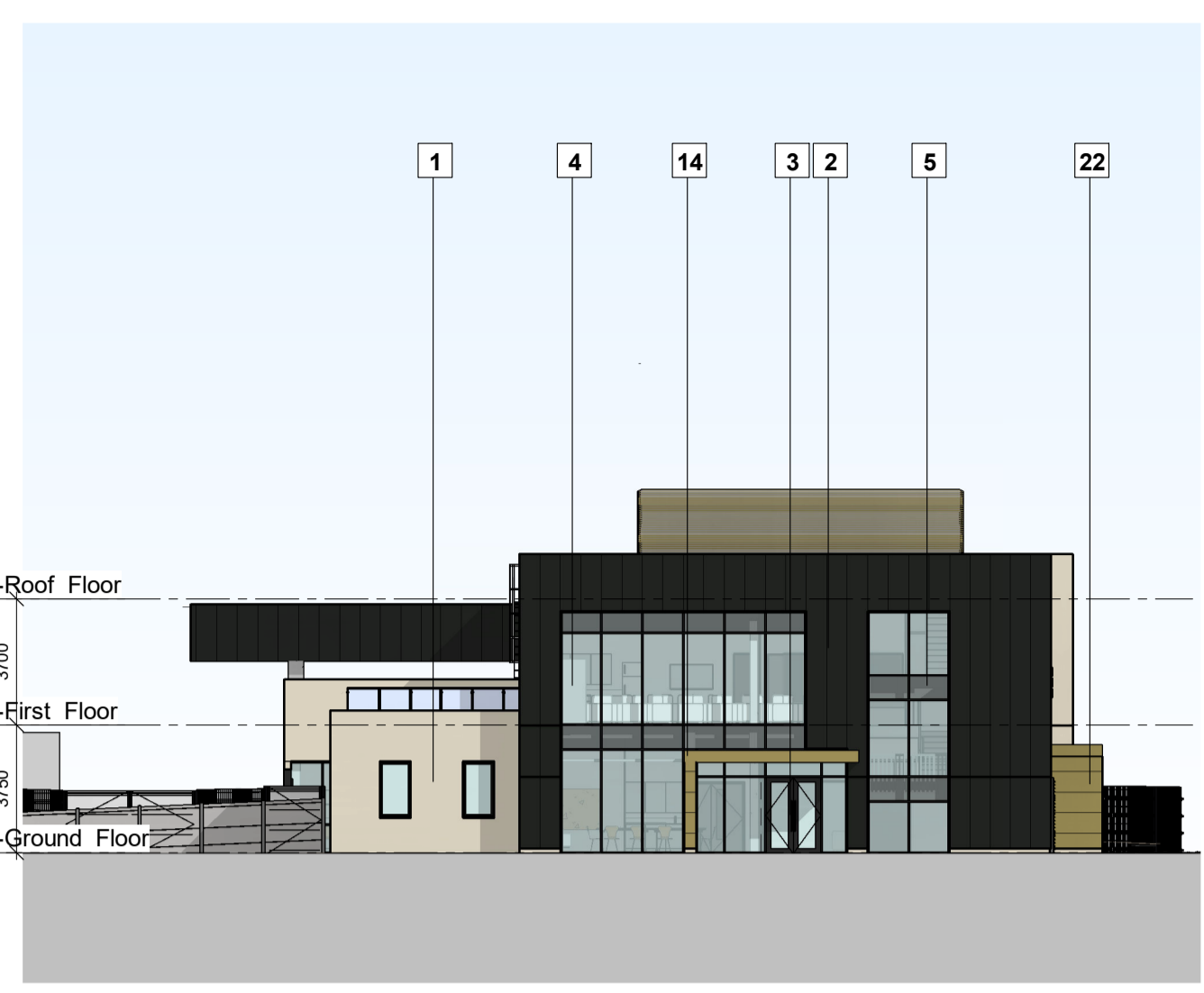
1 Elevation North 1:200
